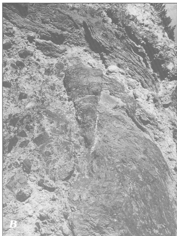
Figure 22. Flow-front breccia exposed in Firehole Canyon. A , Rounded blocks of chilled lava in matrix of smaller rock and glass fragments and B , detail of flow-banded magma within breccia showing fluidal layers locally arrested in process of brecciation.
