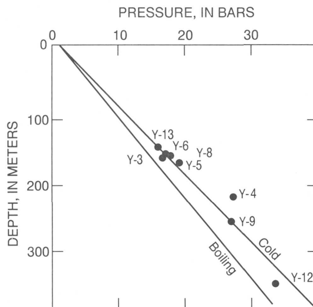
Figure 8. Measured pressure versus depth in U.S. Geological Survey research wells drilled in Yellowstone National Park. Also shown for reference is calculated ideal hydrostatic pressure resulting from weight of a column of cold water extending up to land surface compared to ideal hydrostatic pressure resulting from weight of a column of boiling water. (From Fournier, 1983).
