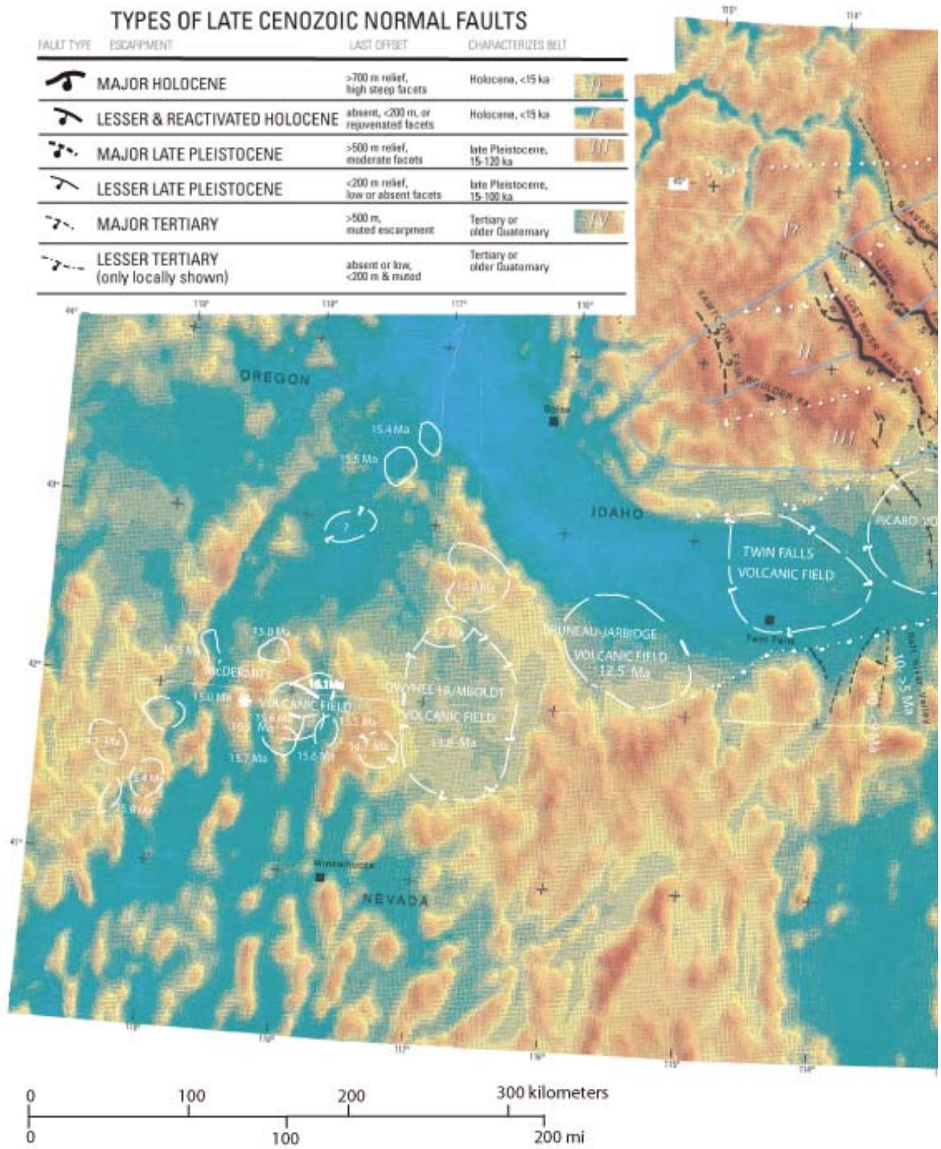
Figure 3 ( continued on facing page ). The track of the Yellowstone hotspot is plotted on a color-shaded topographic relief map of region including the Snake River Plain and Yellowstone Plateau (Pierce and Morgan, 1992, Plate 1).
